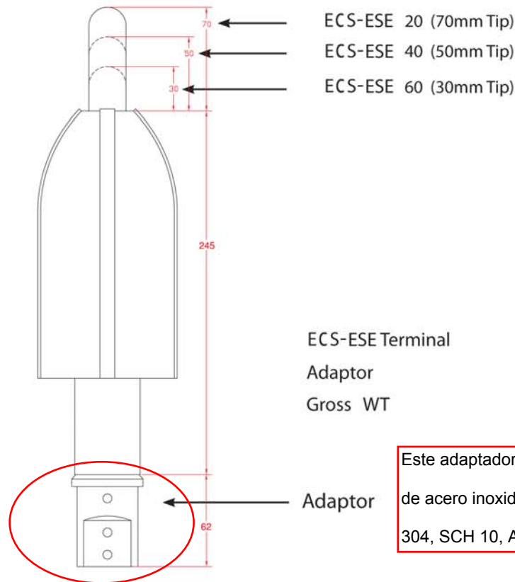
ECS-ESE Terminal (Model ECS-ESE 60/40/20)
